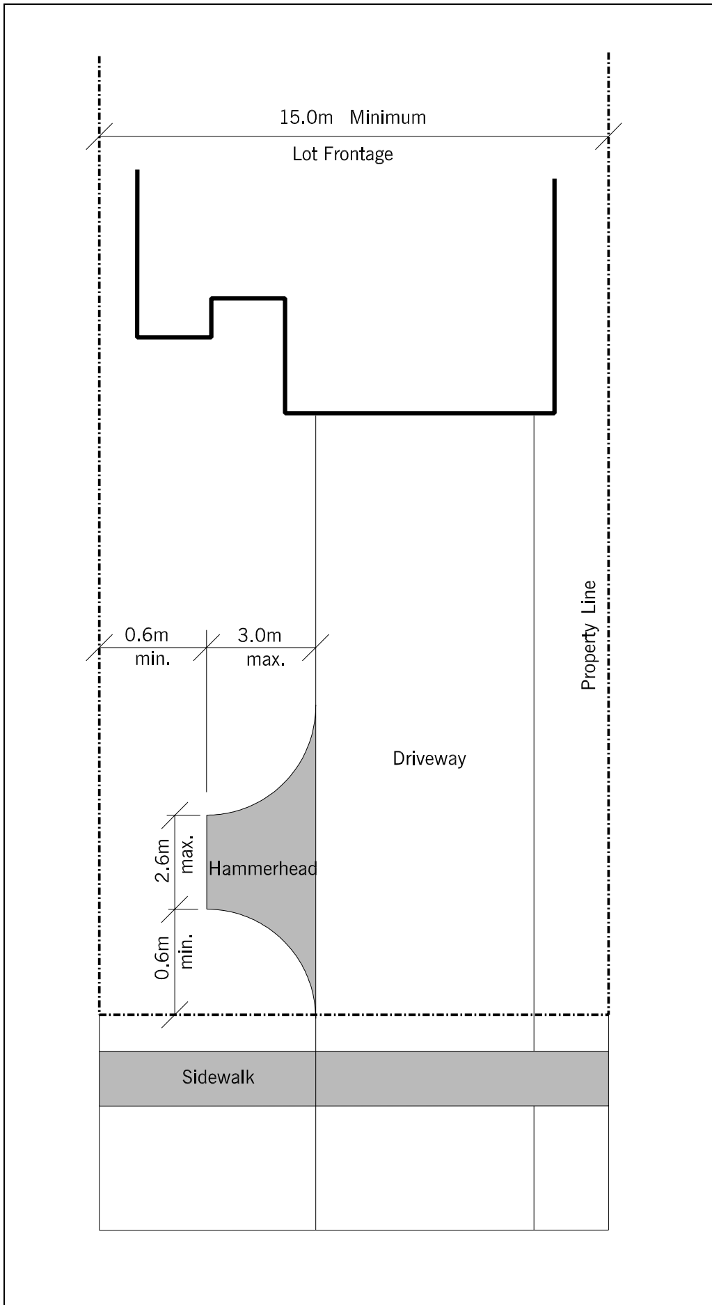
Illustration No. 5 TYPICAL HAMMERHEAD CONFIGURATION
